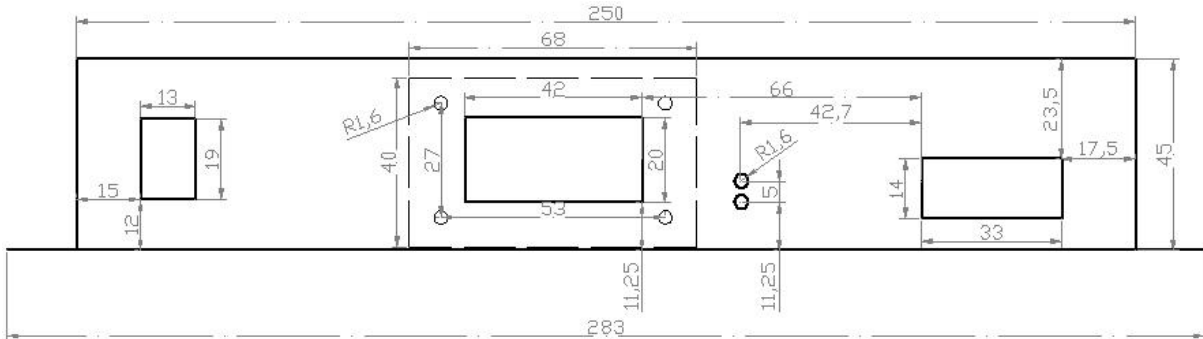
MR-228DW Top View:
