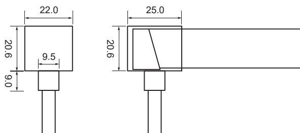
Bottom Entry Connector MJ-SFW20-D3-B02SM MJ-SFW20-D3-B03SFM
