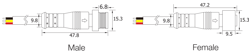
Male & Female Connector SYZ-M12-M-2C-075-W SYZ-M12-F-2C-075-W
