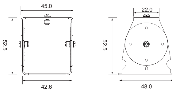
Angle Adjustable Bracket WJJ-CYJ-033
