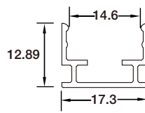
Aluminum Mounting Channel ALCP01S01
