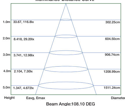
Illuminance-Distance Curve
